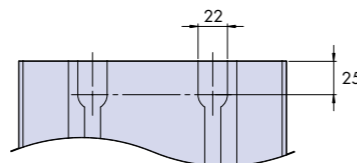
General T-slot Window Details*2
