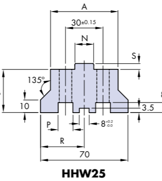
High Wide Back Plate
